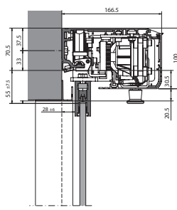
With FAAC glass clamp system
