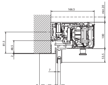
With reduced section profiles FAAC TK20
