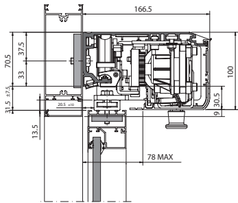
With commercial profiles
