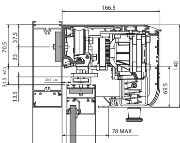
With commercial profiles
