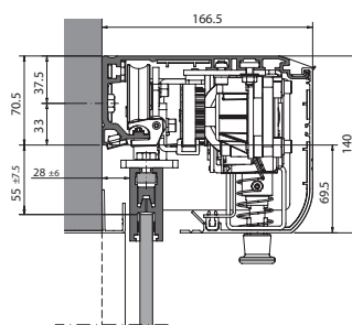
With FAAC glass clamp system
