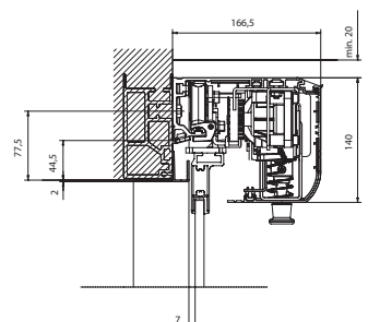
With reduced section profiles FAAC TK20
